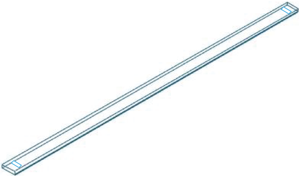
Top Cover 3/16" Clear Acrylic with Polished Edges 21 5/8" x 1/2" x 3/16" 2 small clear acrylic rods applied to bottom to keep in place, exact position TBD
